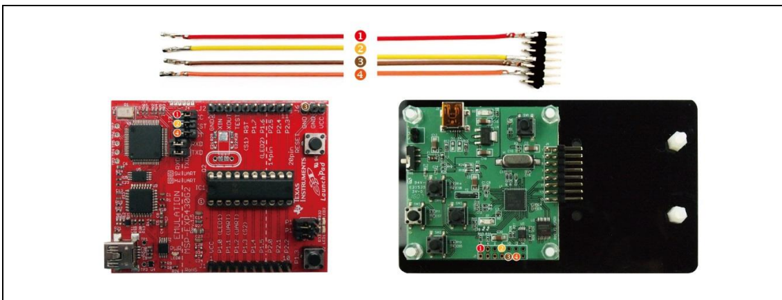
Connect to MSP430 and THOR MCU board
